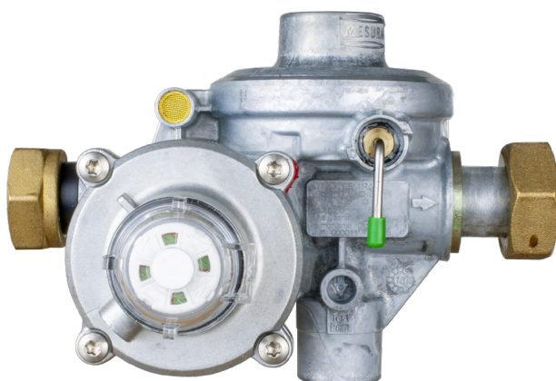
Active Gas Flow - Regulator in use: Indicator in green position
