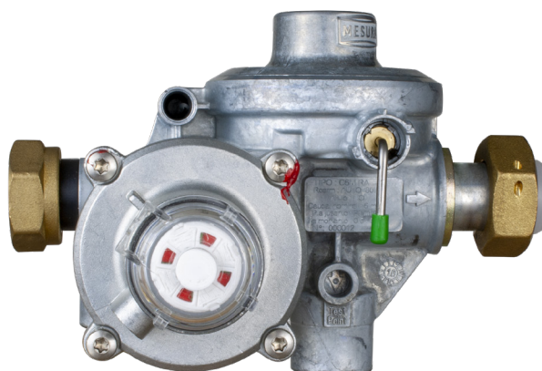
Gas Flow Stopped - Regulator out of order: Indicator in red position
